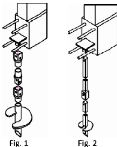
Typical Installation of New Construction Brackets
